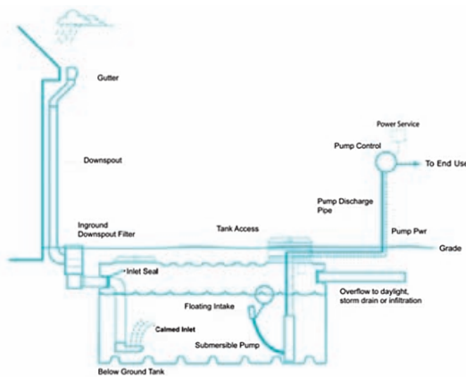
Figure 12: Underground ground storage design
