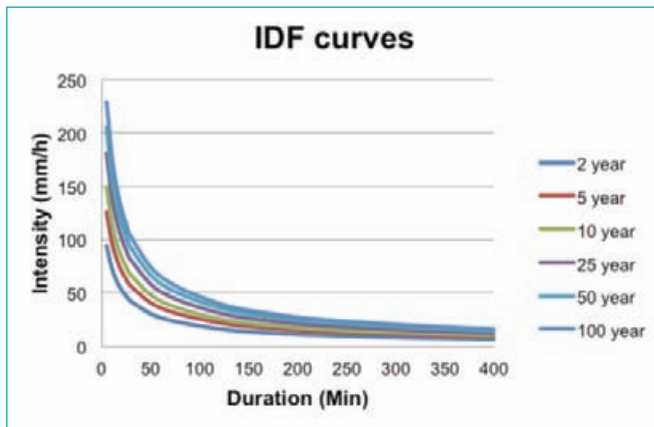
Figure 6: IDF Curves for Lebanon (Provided by Dr. Nadim Farajalla)
