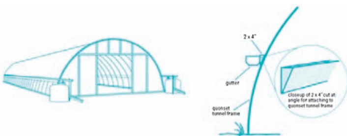
Figure 7: Gutter support board mounted on Quonset (tunnel) greenhouse
