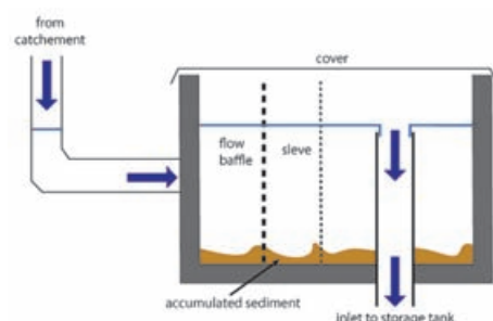
Figure 10: Baffle tank design.
