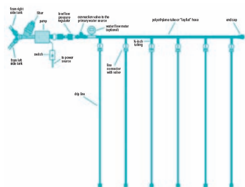
Figure 15: Drip irrigation system main components
