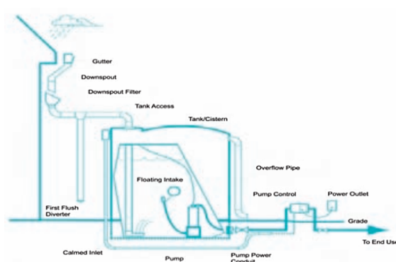
Figure 11: Above ground storage design
